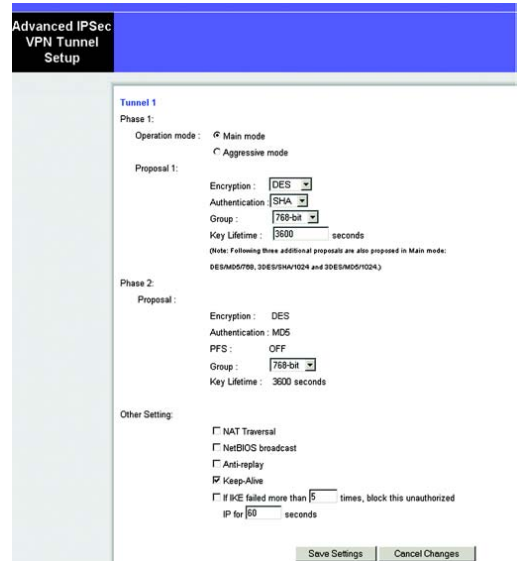
Figure 4-31: Advanced VPN Tunnel Setup
