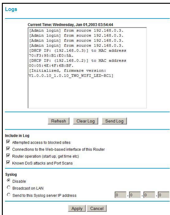
Figure 31. Logs screen
