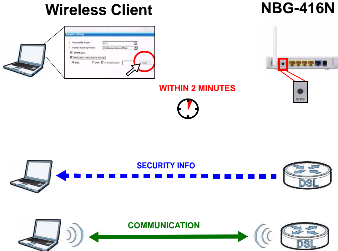
Figure 30 Example WPS Process: PBC Method
