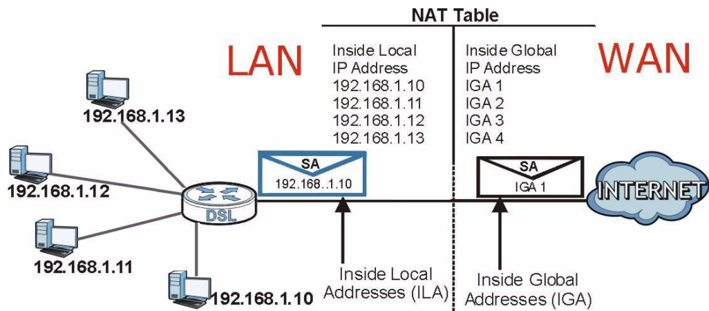
Figure 60 How NAT Works
