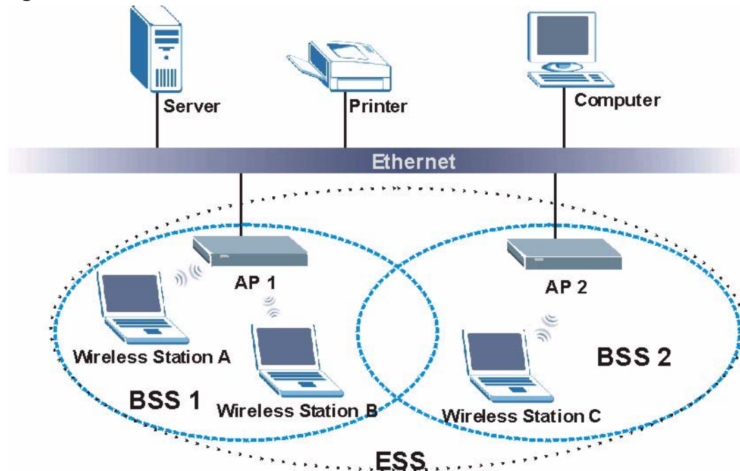
Figure 131 Infrastructure WLAN
