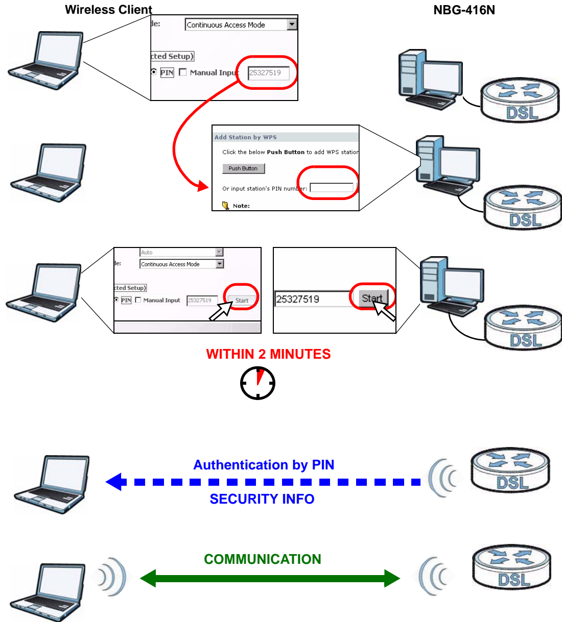
Figure 31 Example WPS Process: PIN Method
