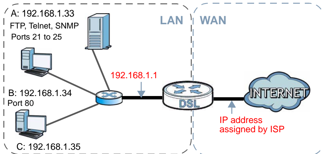
Figure 59 NAT Example
