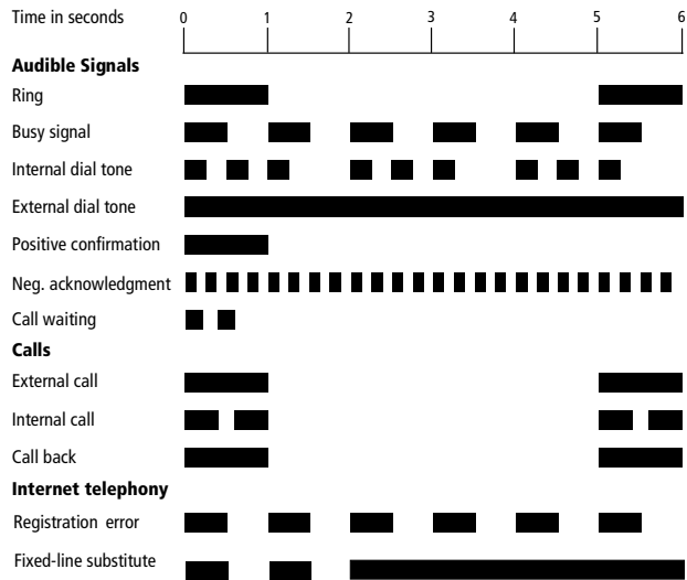
Handset and ring patterns on FRITZ!Box Fon WLAN 7570 vDSL
