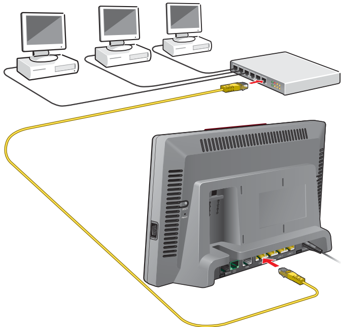
Connecting FRITZ!Box to a network hub
