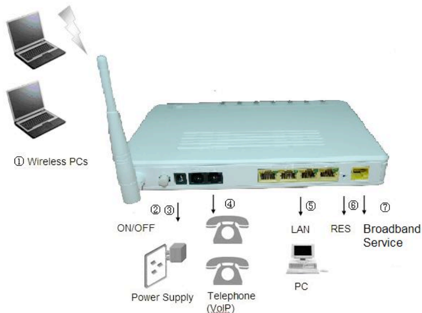
Figure 4: Overview of Hardware Connections for EG101
