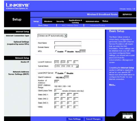
Figure 5-2: Setup Tab - Basic Setup
