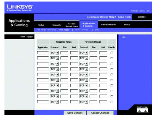
Figure 5-15: Applications & Gaming Tab - Port Trigger
