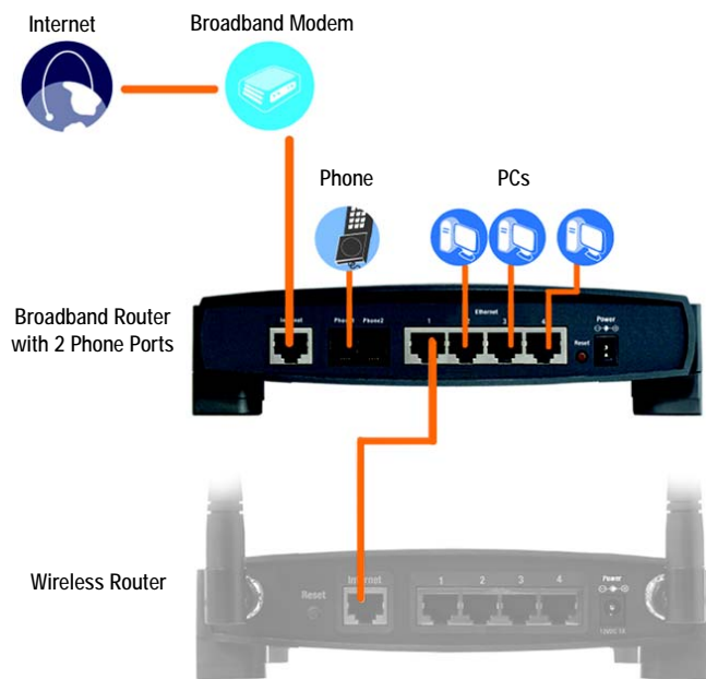
Figure 4-5: Router Connected to Another Router
