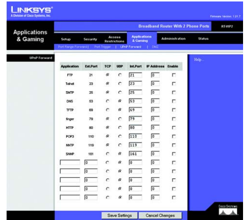
Figure 5-16: Applications & Gaming Tab - UPnP Forward
