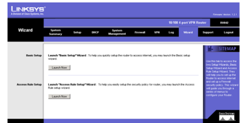
Figure 6-50: Wizard
