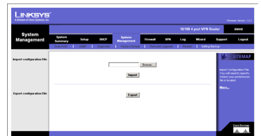
Figure 6-32: Setting Backup
