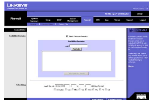
Figure 6-39: Content Filter
