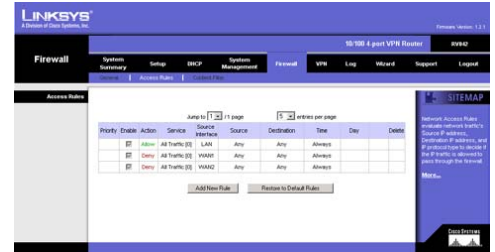
Figure 6-35: Access Rules
