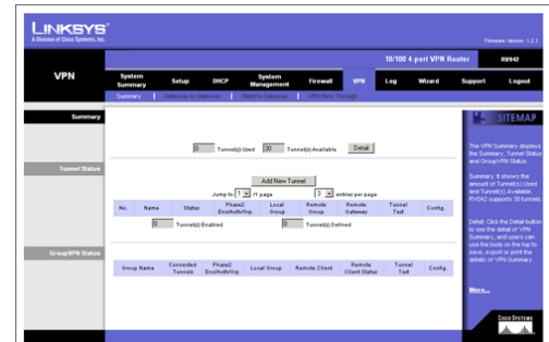
Figure 6-40: VPN Summary
