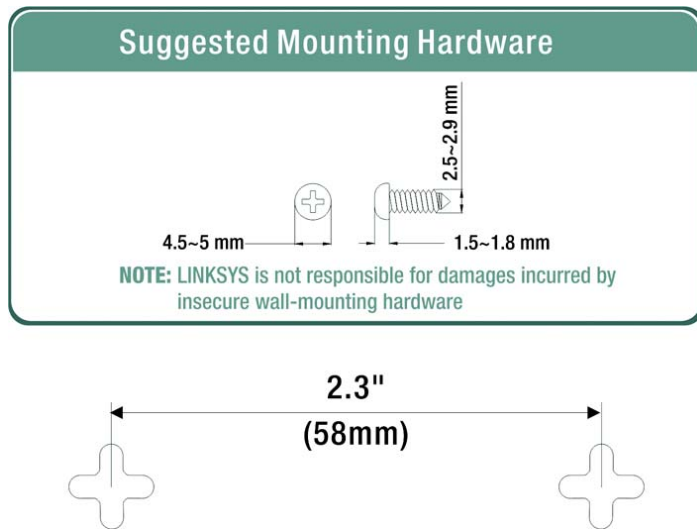
Figure D-1: Wall-Mounting the Router
