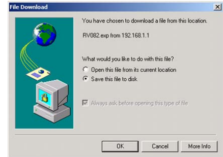
Figure 6-33: Save File
