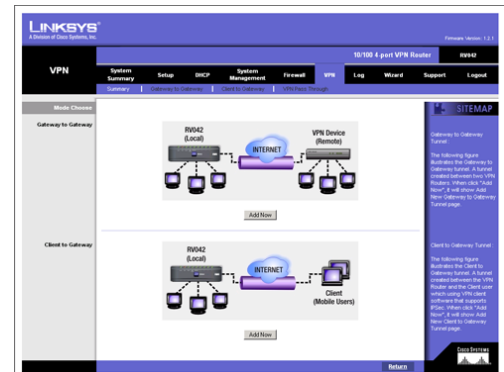
Figure 6-41: Mode Choose
