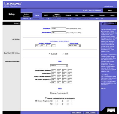
Figure 6-5: Setup Tab
