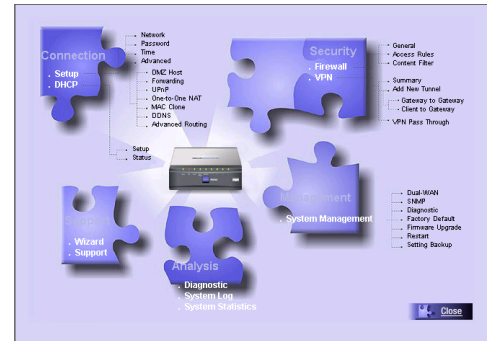
Figure 6-4: Site Map
