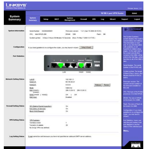
Figure 6-3: System Summary
