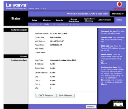
Figure 8-60: Status Tab - Router
