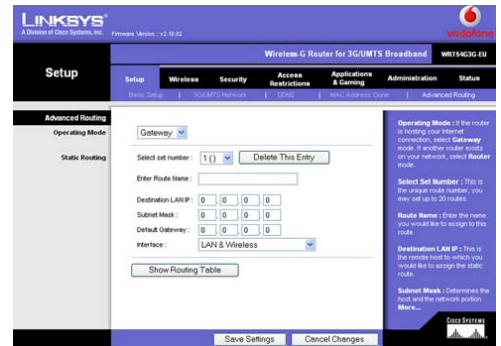
Figure 8-21: Setup Tab - Advanced Routing (Gateway)
