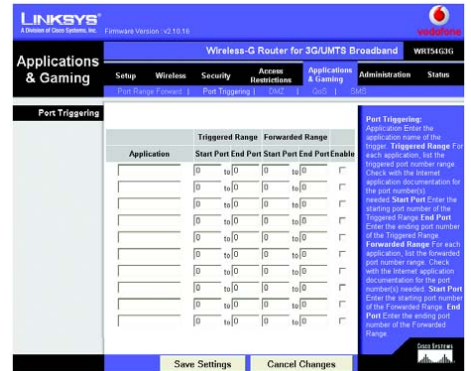
Figure 8-46: Applications and Gaming Tab - Port Triggering
