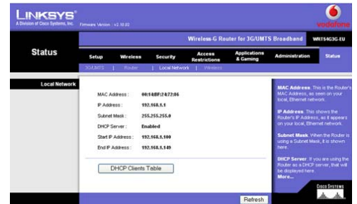
Figure 8-61: Status Tab - Local Network
