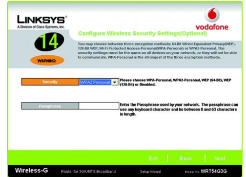
Figure 7-25: Configure Wireless Security Settings - WPA2-Personal Screen
