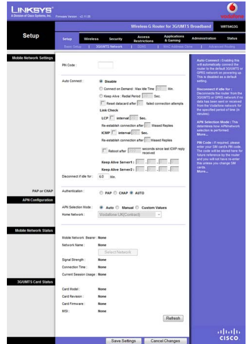
Figure 8-15: Setup Tab - 3G/UMTS
