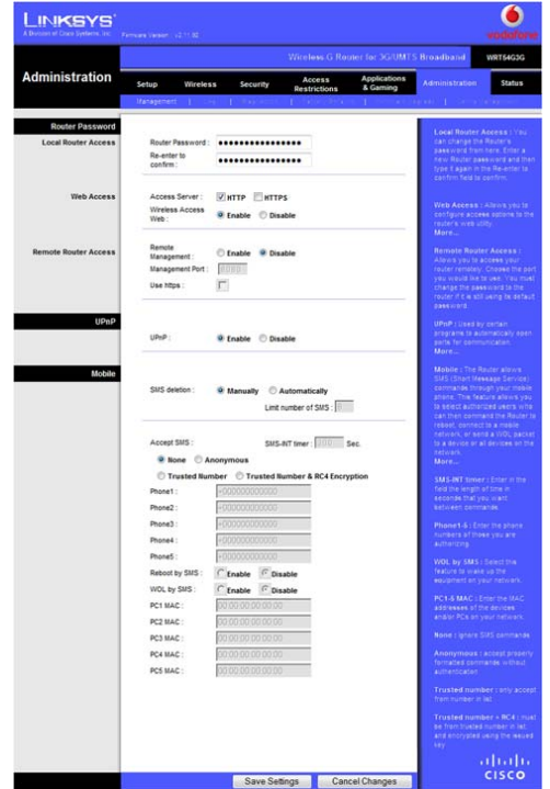
Figure 8-51: Administration Tab - Management
