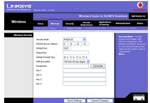
Figure 8-32: Wireless Tab - Wireless Security (RADIUS)
