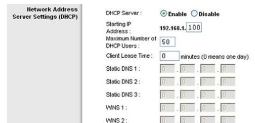
Figure 8-13: Network Address Server Settings
