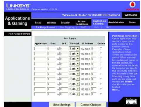
Figure 8-45: Applications and Gaming Tab - Port Range Forward
