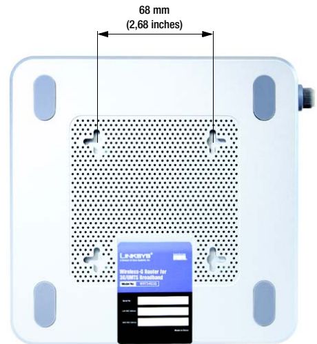
Figure 4-11: Measurement between Wall-Mount Slots
