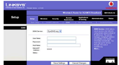
Figure 8-18: Setup Tab - DDNS (DynDNS.org)
