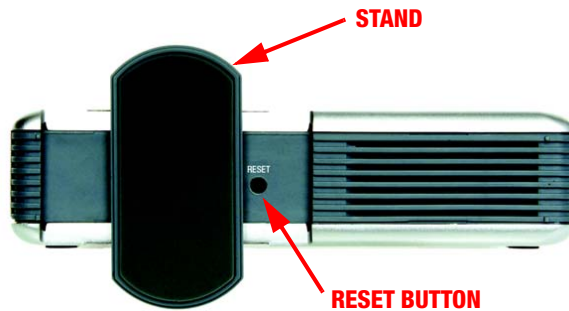
Figure 3-3: The Router's Bottom Panel
