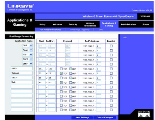
Figure 5-30: Applications and Gaming Tab - Port Range Forwarding
