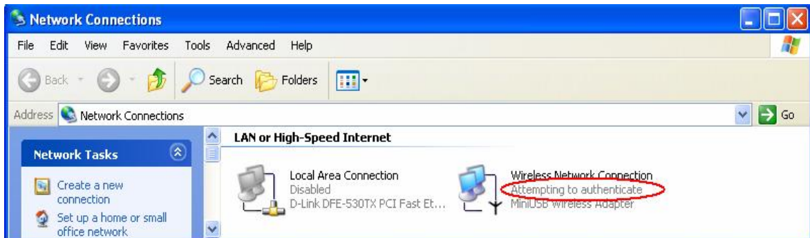
Figure 5: Authenticating
