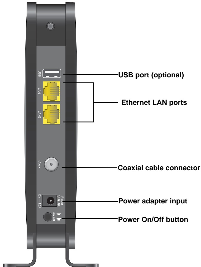
Figure 3. Modem router rear panel
