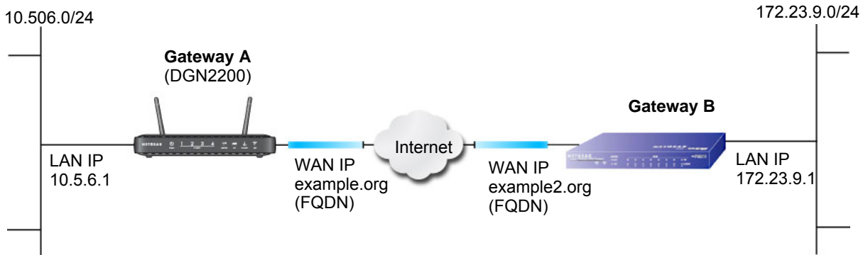
Figure 29. VPNC Example, Network Interface Addressing
