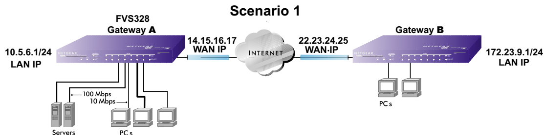
Figure 7-6: LAN to LAN VPN access from an FVS328 to an FVS328
