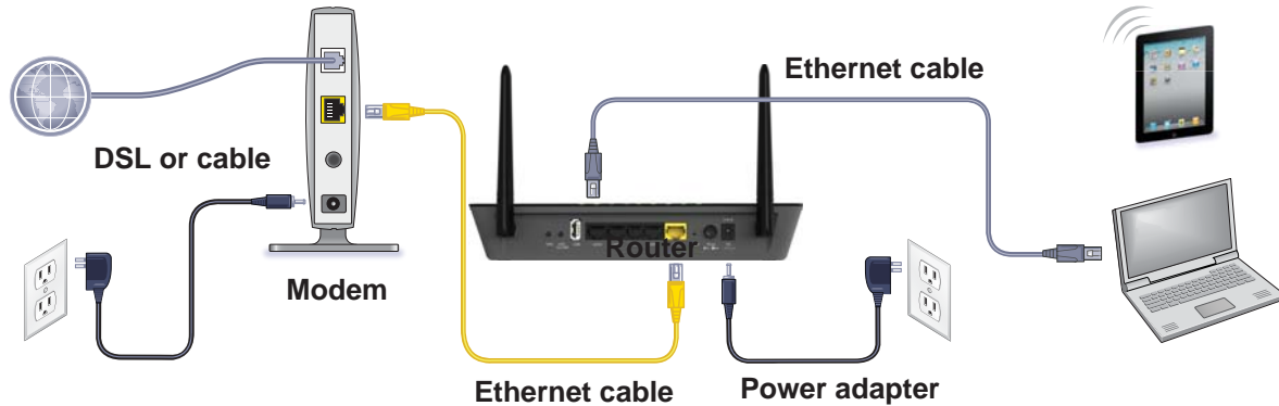
Figure 3. Router cabling
