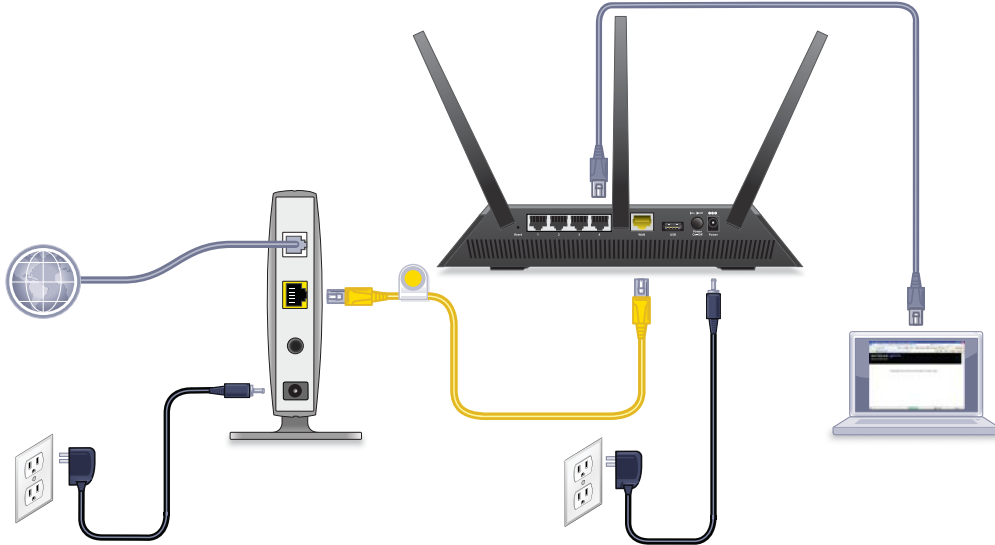
Figure 4. Router cabling
