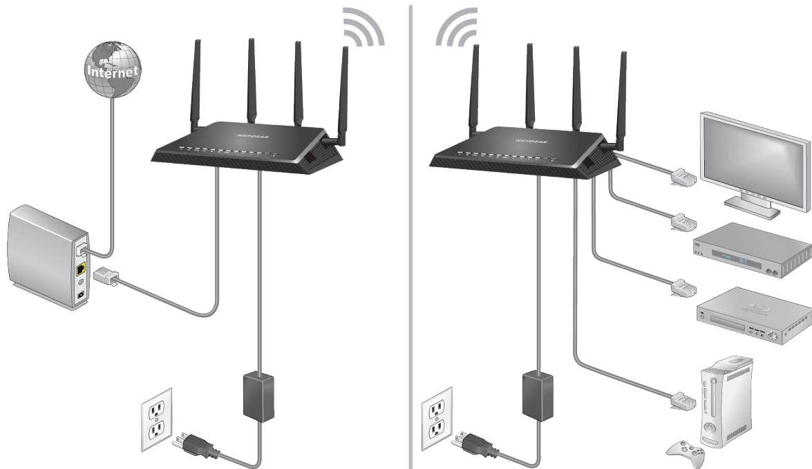
Figure 7. Router in bridge mode with an 802.11ac WiFi connection
