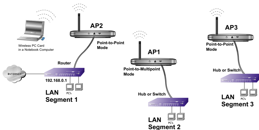
Figure 5-4: Wireless Bridging
