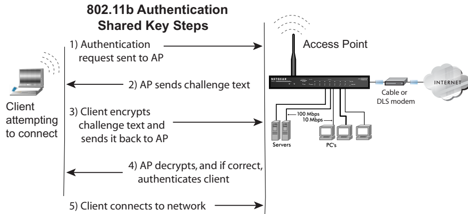
Figure C-2: 802.11 shared key authentication
