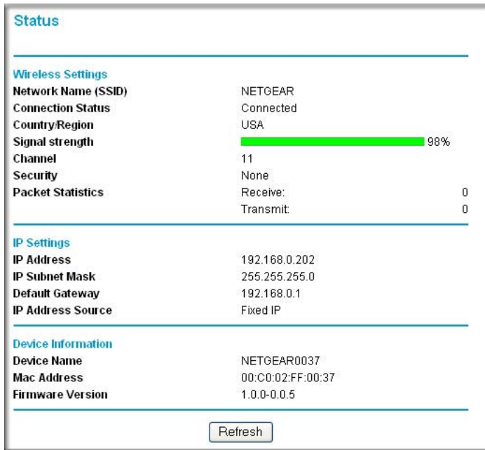
Figure 4-1: Status screen
