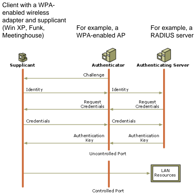
Figure C-4: 802.1x Authentication Sequence
