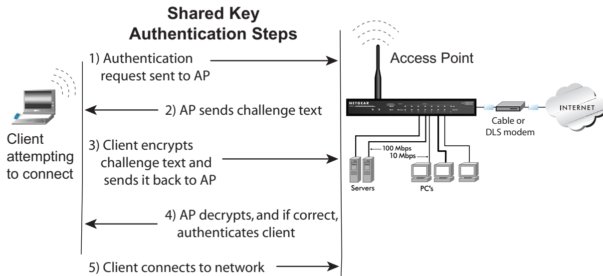
Figure 7-5: Shared key authentication
