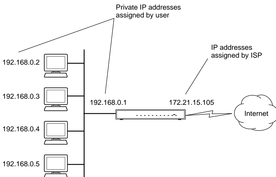
Figure 7-3: Single IP Address Operation Using NAT
