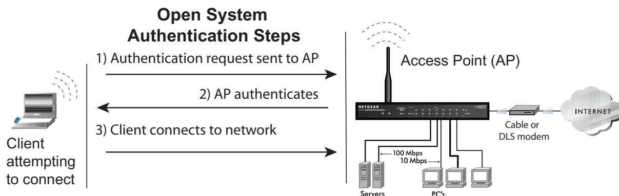
Figure 7-4: Open system authentication
