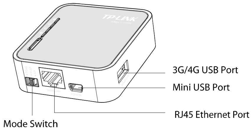
Figure 1-2 Rear Panel sketch
