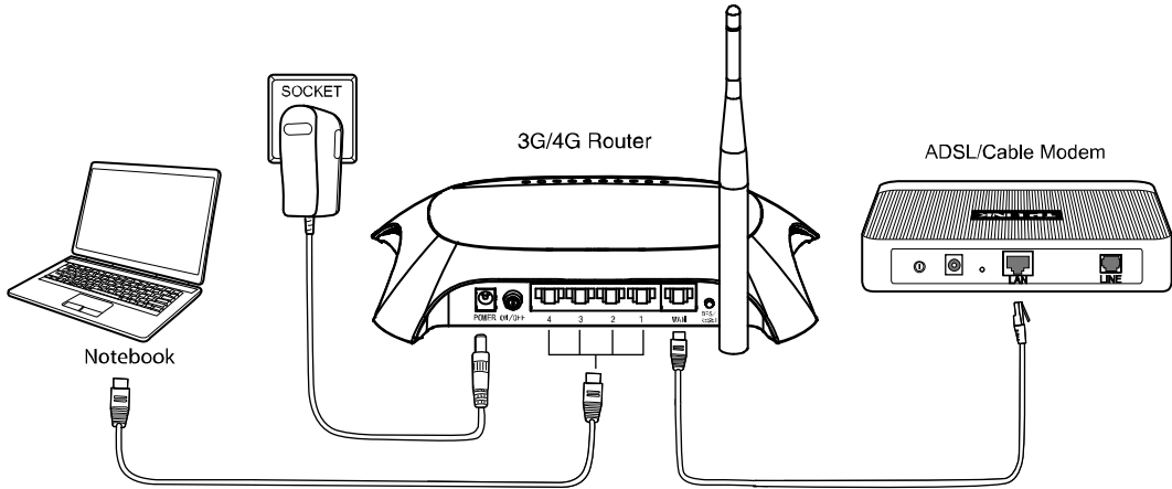
Figure 2-2 Hardware Installation of the 3G/4G Wireless N Router – WAN connection
