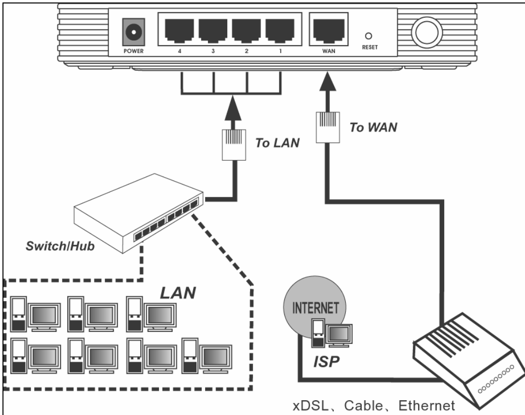
Figure 2-1 Hardware Installation of the TL-WR642G 108Mbps Wireless Router
