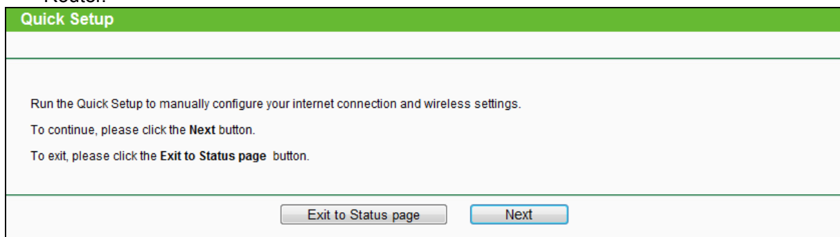
Figure 3-4 Quick Setup
