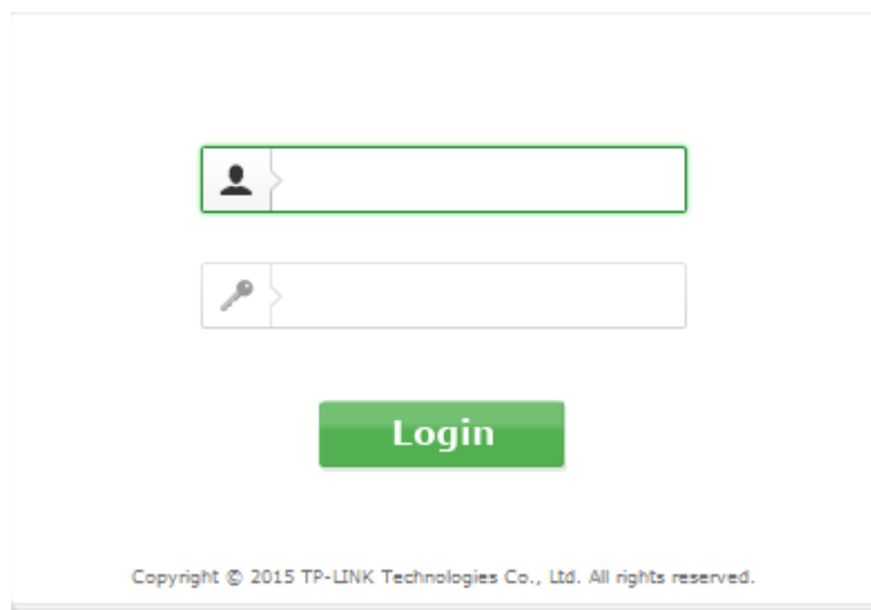
Figure 3-3 Login Windows
