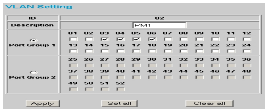
Figure 20. VLAN Settings
