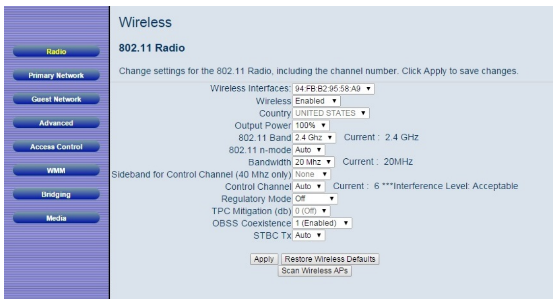
Figure 30. Example of Radio Page
