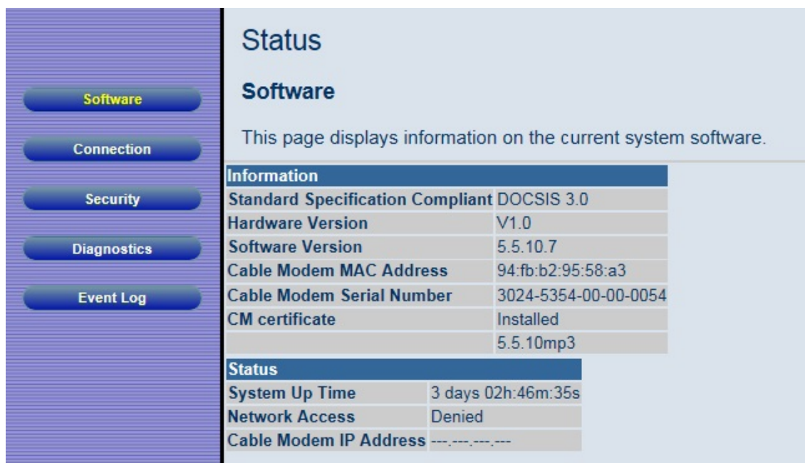
Figure 4. Software Menu
