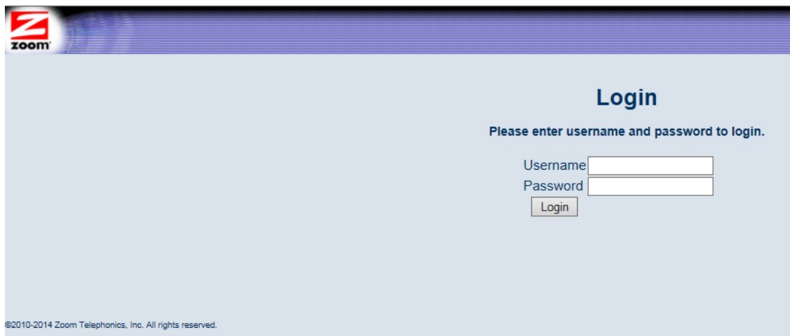
Figure 1. Login Screen
