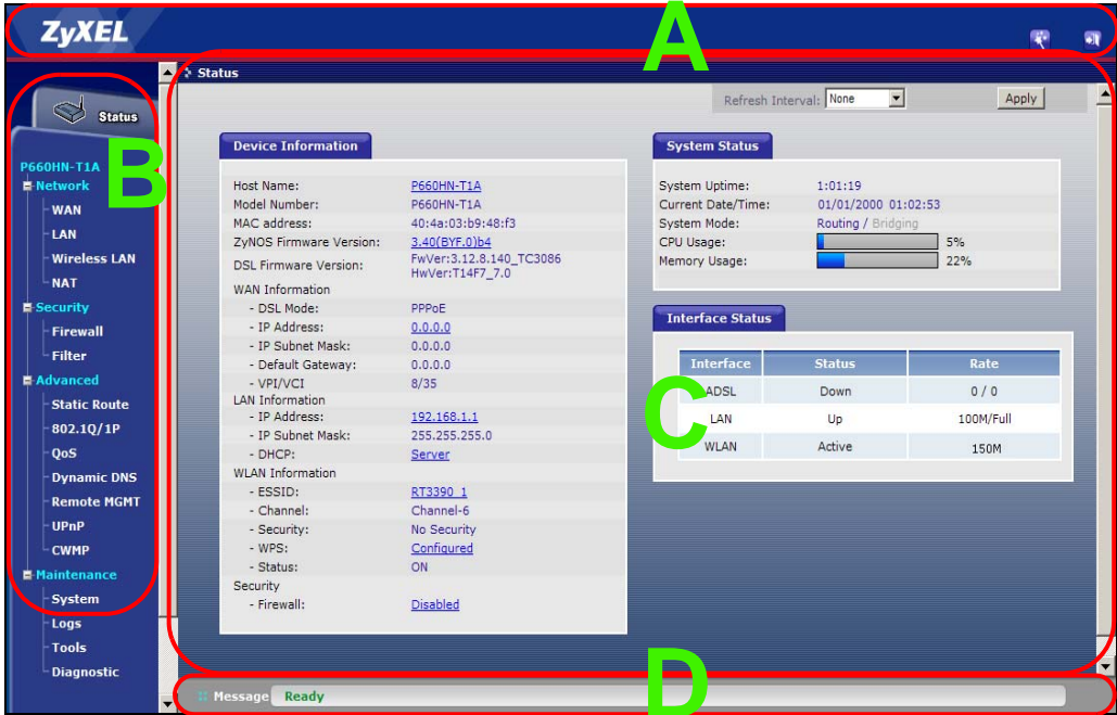
Figure 7 Main Screen
